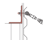
METAL BUILDING
